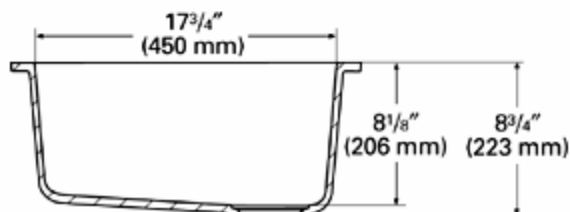
Side Cross-Section
